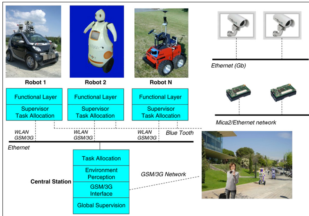
Fig. 1. URUS architecture.
